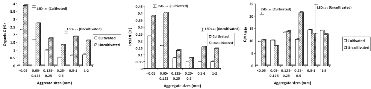
Figure 5 : Topsoil (0-15 cm) distribution of (a) organic C, (b) total N and (c) C:N in aggregate size fractions as influenced by cultivation
