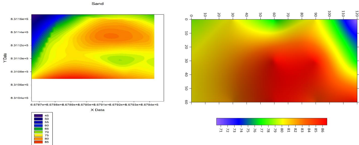
Fig 13: Spatial distribution of soil sand content in the OAU main football field in (a) 2019 and (b) 2025.
