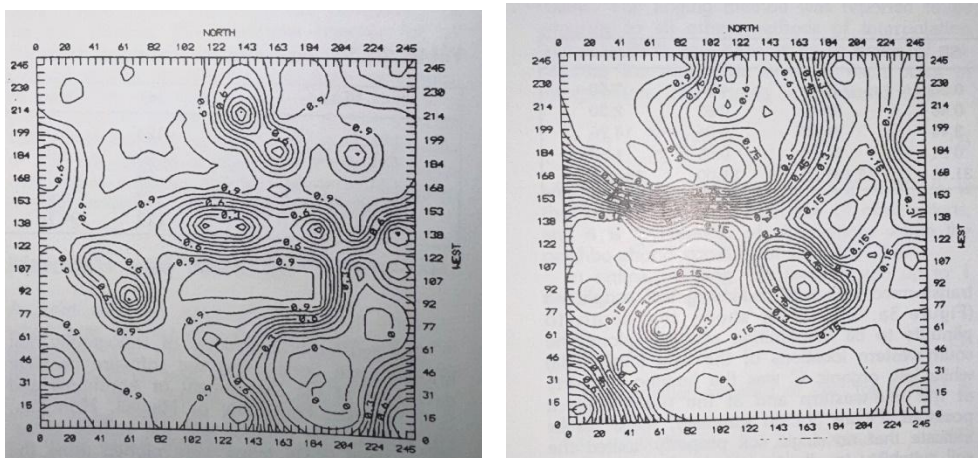
Figure 7: Isarithmic map of % gravel for (a) Kriged estimates and (b) actual samples
